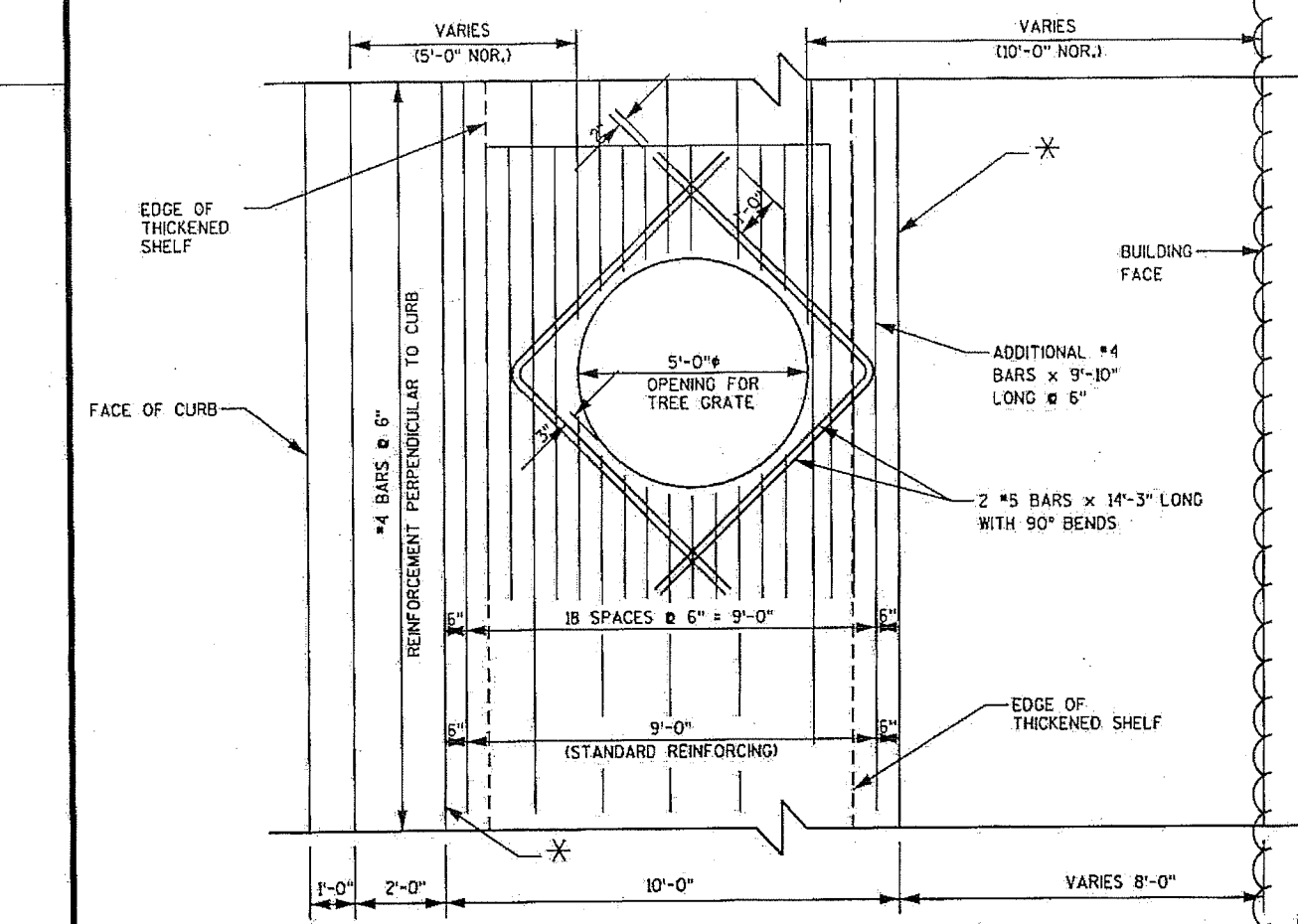
REINFORCEMENT PLAN - TREE OPENINGS
