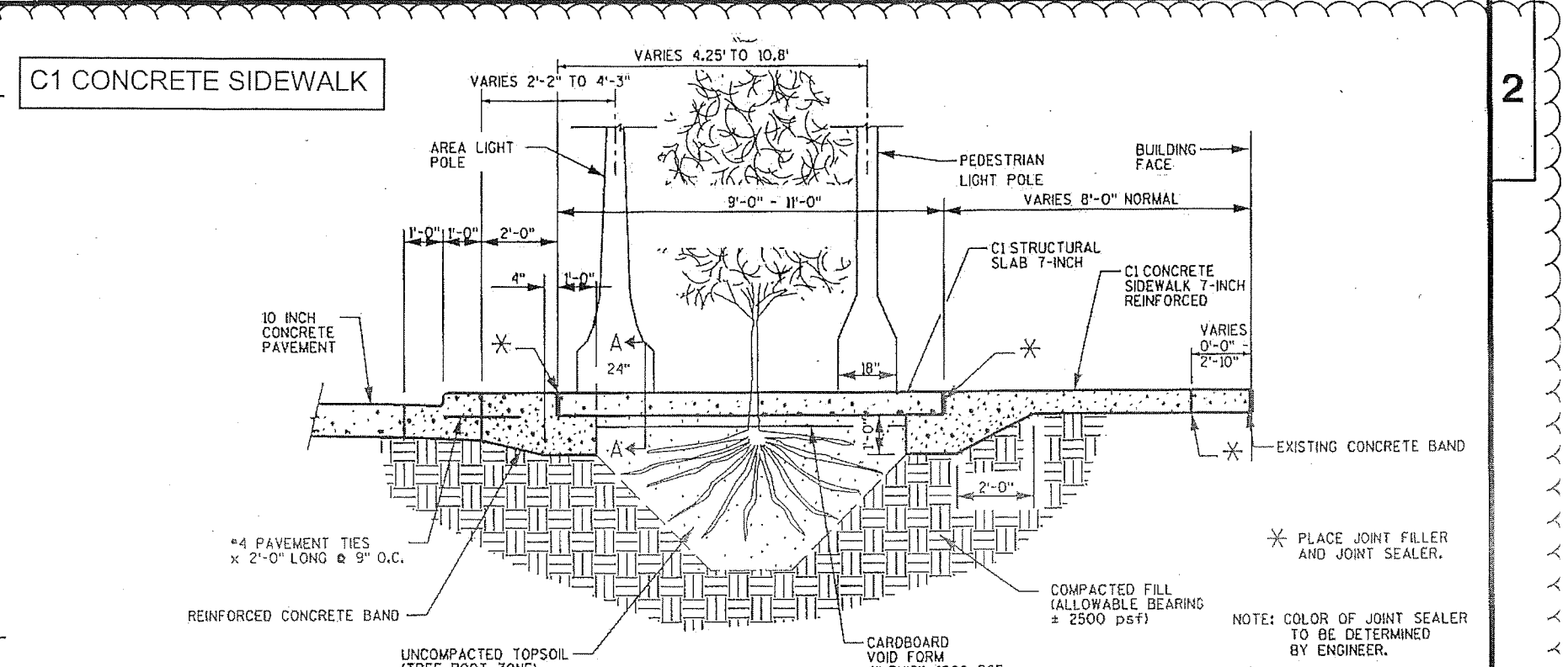
ROOT ZONE DETAIL
