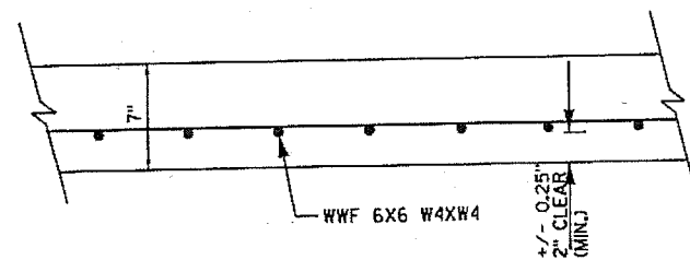
C1 CONCRETE SIDEWALK 7-INCH MESH REINFORCED
