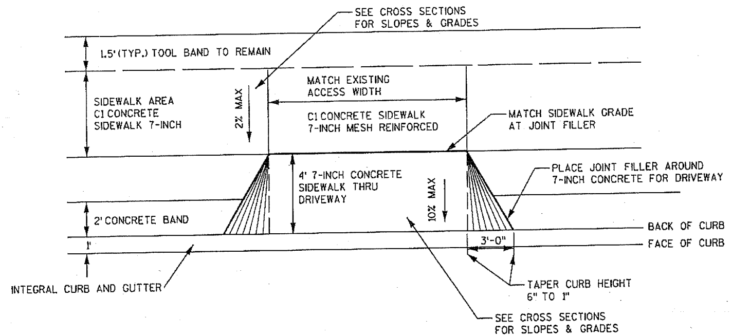
DRIVEWAY DETAIL
