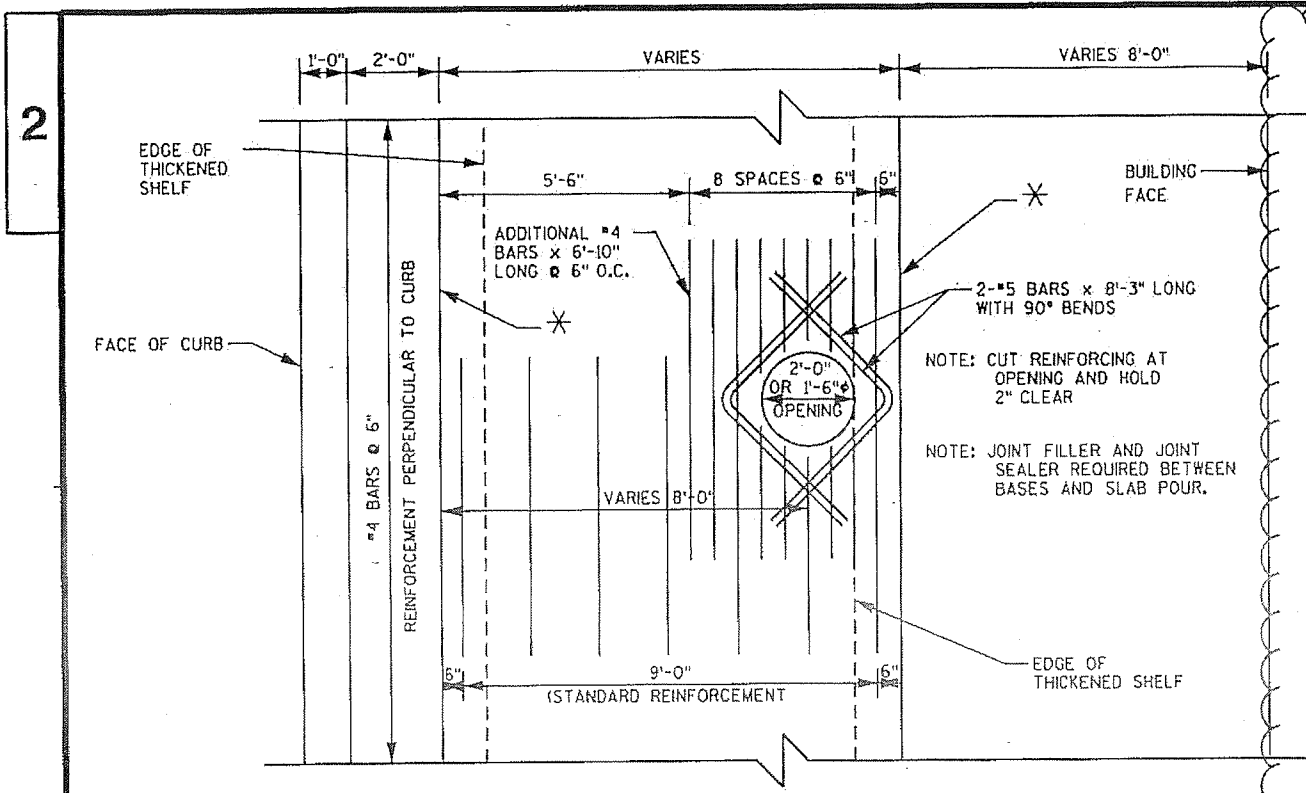
REINFORCEMENT PLAN - LIGHT BASE OPENINGS
