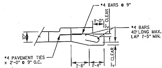
REINFORCED CONCRETE BAND
