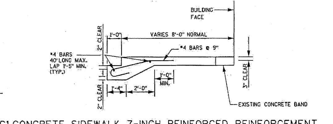
C1 CONCRETE SIDEWALK 7-INCH REINFORCED REINFORCEMENT
