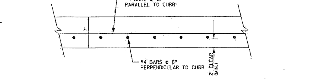
SECTION A-A, C1 STRUCTURAL SLAB 7-INCH REINFORCEMENT
