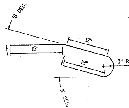
REINFORCED CONCRETE BAND REINFORCEMENT
